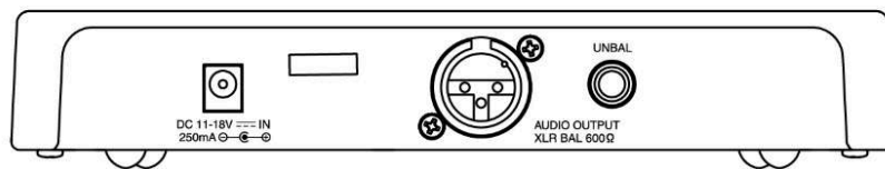
Rear View
